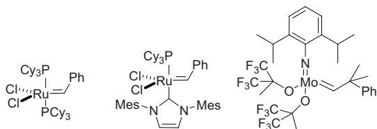
Grubbs' catalysts
